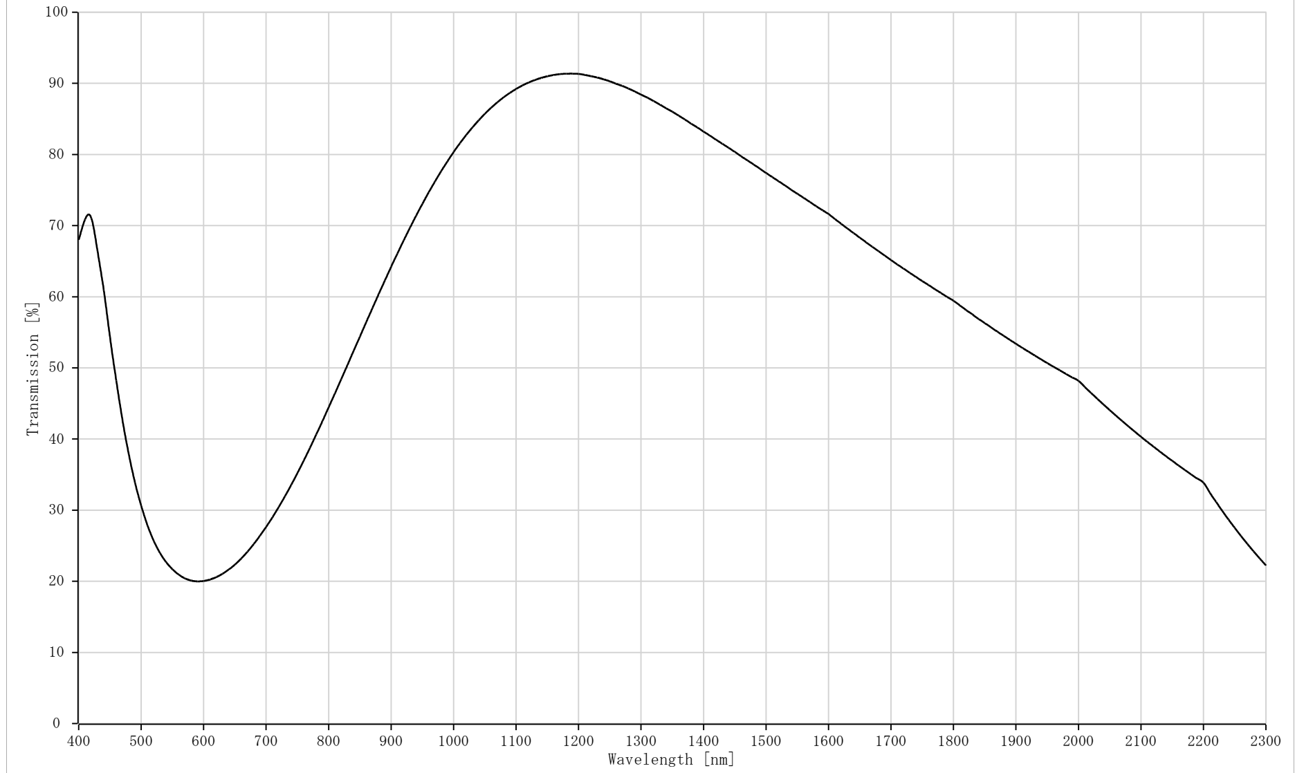
LM6HC-SW Transmission
